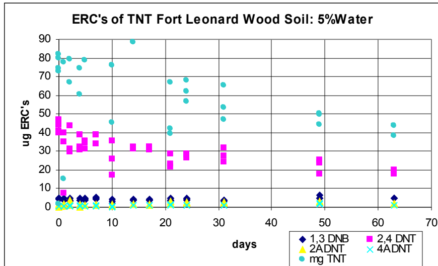
Figure 3 Changes in TNT & ERC's Concentrations in Fort Leonard Wood Soil Moistened with 5% Water
