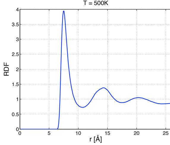
FIG. 16: Radial distribution function of a NPT simulations with 504 molecules at pressure of 1 bar and temperature of 500°K.
