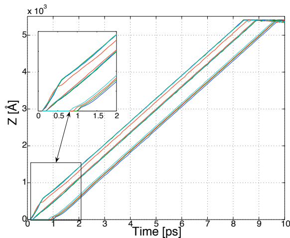
FIG. 2: Reaction front location versus time in simulations with three different initial velocities of the pellet. The location was determined by a significant dissociation ratio. The results are grouped in three categories: The rightmost bundle represents five different simulations with the lowest pellet velocity used ( \approx 10 km/s). The central bundle corresponds to simulations (5 runs) with medium pellet velocity ( \approx 50 km/s), while the leftmost bundle corresponds to simulations with the largest pellet velocity ( \approx 120 km/s). (These high values of initial velocities are used for demonstration: pellet velocities of 10, 50, and 120 km/s give rise to initial transient shock waves that are, respectively, slower, similar, and higher than the developing stable detonation wave. Smaller values of pellet’s velocities will be used subsequently). The different simulations in each one of the three groups correspond to different initial conditions used (slightly different initial pellet-crystal distance). A short time after the pellet collision with the slab, different shock wave velocities develop in each simulation. The differences between the trajectories at short times are shown in the insert of the figure. A stable, steady state, velocity is reached after an additional propagation period. The shock velocity depends only on crystal parameters, which are identical in all simulations.
