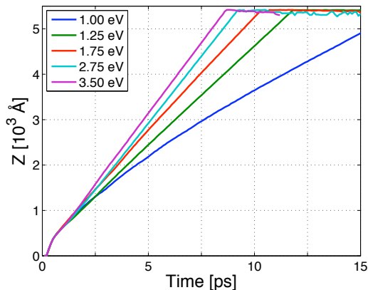
FIG. 10: Reaction front propagation in crystals with different exothermicity values. All other parameters are identical.
