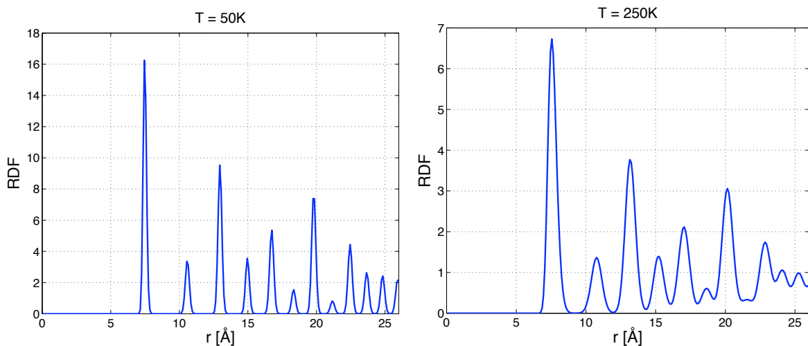
FIG. 15: Radial distribution function of the crystal. Results are of a NPT simulations with 504 molecules at pressure of 1 bar. The left plot corresponds to 50°K, and the right corresponds to 250°K.
