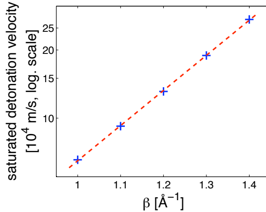
FIG. 14: Comparison of reaction propagation velocities (scaled logarithmically) in 5 different crystals, \beta ranges from 1 \text{\AA}^{-1} to 1.4 \text{\AA}^{-1} (when \beta is the coefficient inside the Morse potential's exponent). The exponential dependence suggests that the saturation of the detonation velocity is caused by the repulsive part of the intermolecular potential. This is different from the elastic p-wave velocity dependence, which is governed by the behavior of the potential near the equilibrium point (see appendix C2 b and Fig. 17).
