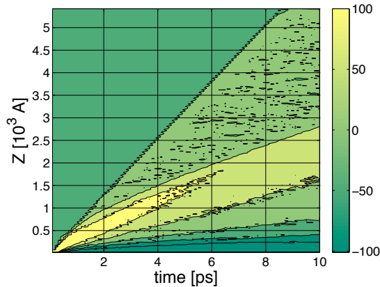
FIG. 5: Contour plot of mass velocity along the Z direction. The dissociation barrier height in this simulation was 0.25\text{ eV} , and the reaction exothermicity was 6\text{ eV} . The initiating pellet velocity was \sim 7\text{ km/s} . The mass velocity plot shown here can be compared to the decomposition percentage during the same simulation, which is shown on the right plot of figure 4: The decomposition front and the discontinuity of the mass velocity coincide, characterizing the reaction wave. The compression wave is visible on the mass velocity plot, but is almost absent on the decomposition plot: For this barrier height, most of the molecules have already decomposed before the compression wave reached them.
