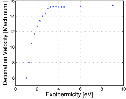
FIG. 11: Detonation velocity in the crystal as a function of reaction exothermicity. The detonation velocity is measured in reduced units, normalized to the p-wave velocity. We can see the increase of detonation velocity as a function of exothermicity at low exothermicity values, until approximately 3 eV. The saturation of the detonation velocity at high exothermicity values can also be seen. The saturation was verified by simulations with very high exothermicity values: there is a very small increase of the detonation velocity in crystals with higher exothermicity values (12 eV, 15 eV, 18 eV, and even 27 eV. These results are not shown here).
