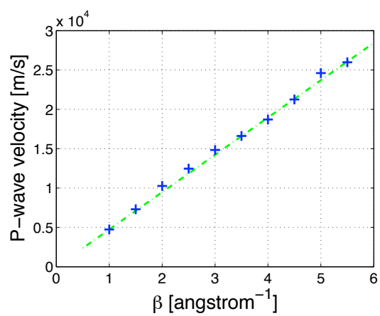
FIG. 17: P-wave velocity in the crystal as a function of the \beta parameter in the intermolecular Morse potential. Each velocity was calculated by simulating propagation of small displacements in a crystal, with the relevant \beta parameter, and marked in the figure by a cross. The dashed line is an extrapolation to small \beta values assuming linear scaling.
