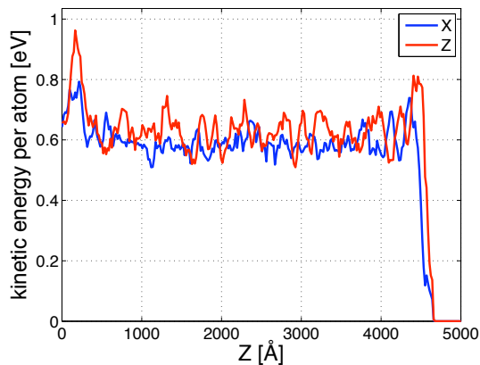
FIG. 7: Normalized kinetic energy profile at time = 10\text{ ps} . The exothermicity of the reaction in this simulation was 6\text{ eV} , and the dissociation barrier was 0.25\text{ eV} . The values were averaged over bins with constant number of particles, 96, in each bin. The blue line corresponds to kinetic energy along the X direction, and the red line to kinetic energy along the Z direction. The large peak on the right corresponds to the reaction wave front.
