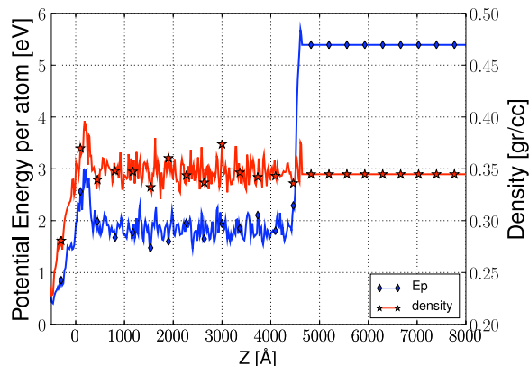
FIG. 9: Potential energy ( E_p ) and density profiles at t = 10 ps. The parameters are the same as in Fig 7. The first shock front displays a small increase of the potential energy, due to a small compression before the dissociation. This small increase is followed by a large decrease of the potential energy, due to the energy release of the exothermic decomposition. The average density after the reaction front is not significantly higher than the density before this front. The peak on the left is associated with the compression wave.
