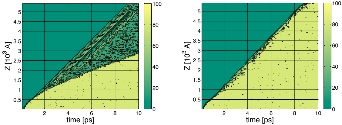
FIG. 4: Contour plots of decomposition percentage during two different simulations. The left plot is obtained in a simulation with a dissociation barrier of 2\text{ eV} . Some of the molecules are decomposed by the reaction wave. Most of the other molecules (around 90%) are decomposed by the compression wave. The right plot is obtained in a simulation with a decreased dissociation barrier of 0.25\text{ eV} . More than 85% of the molecules are decomposed by the reaction wave. In both cases the exothermicity is 6\text{ eV} , and the initiating pellet velocity is \sim 7\text{ km/s} . The shock front velocity is almost independent of the value of the dissociation barrier.
