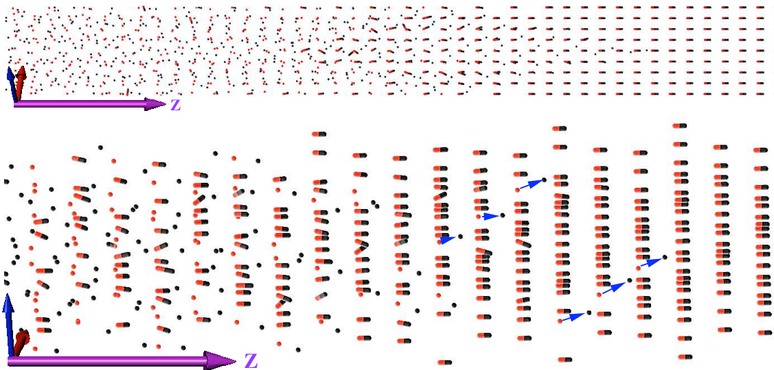
FIG. 3: A snapshot of the detonation wave. The propagation axis is the Z direction. Periodic boundary conditions are used in the X, Y directions. The right hand side shows the unperturbed crystal structure. The red objects represent the heavy particles (N). The black objects represent the light particles (C). On the left side of the image one can observe the burnt material after the passage of the shock wave. The shock front is characterized by pilot cascades of light particles which are emitted from the decomposed molecules, and initiate the next layer in a domino-like effect. The lower panel is an enlarged viewpoint of the detonation front. The arrows indicate decomposed N-C pairs, corresponding to the pilot cascade. This simulation was carried out with exothermicity of 6 \text{ eV} and a barrier of 0.25 \text{ eV} . Eventually, in this simulation, in approximately 20 layers, most of the material is decomposed.
