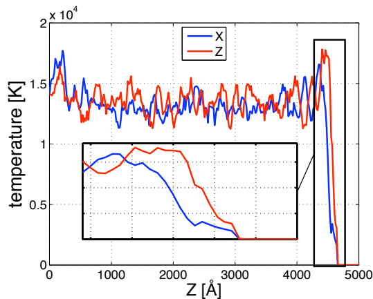
FIG. 8: Local temperature profile at time = 10 ps. The parameters are the same as in Fig 7. The blue line represents temperature along the X direction, and the red line along the Z direction. The insert shows an unthermalized region: The large peak on the right is the reaction wave front. The increase of the Z component of the local temperature precedes the increase of the X direction.
