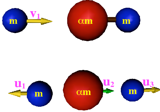
FIG. 12: A molecule is hit by a light particle, emitted from neighboring decomposition (top diagram). After the collision, the molecule decomposes (bottom diagram).
