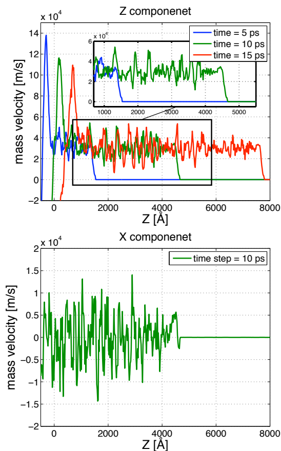
FIG. 6: Mass velocity profiles along Z and X directions. The exothermicity of the reaction in this simulation was 6\text{ eV} , and the barrier was 0.25\text{ eV} . The values were determined by averaging over bins with constant 96 particles in each bin. The left edge of the crystal is placed at -500\text{ \AA} . The top plot shows the profile of the mass velocity in the Z direction, at three time values. The bottom plot presents the mass velocity along the X direction at a single time value. Along the Z direction (top figure), the largest amplitude (the left peak on each time step) is associated with the secondary compression wave. At later times the peak mass velocity decays due to dissipation. The first shock front (the right peak on each time step) is associated with the reaction wave. The reaction wave amplitude does not decay. The insert shows a zoom of the first shock fronts for the two shorter times.
