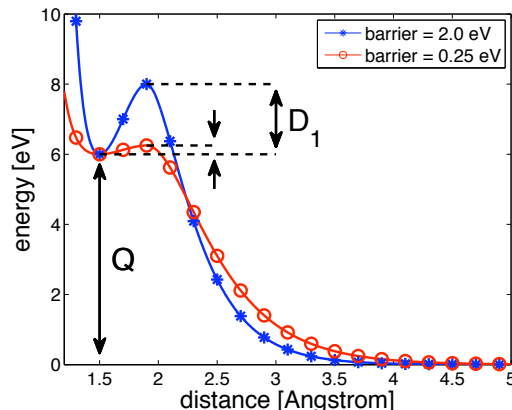
FIG. 1: The reactive internal potential as a function of the N-C distance. for two different ratios between the barrier height and the exothermicity. When the distance N-C is smaller than the barrier position (here at 1.9 Å - the local maximum) the molecule is bound. When the distance is increased beyond this position the molecule dissociates. Initially, the N-C distance is at the equilibrium distance (here at 1.5 Å - the local minimum). Q represents the exothermicity, and D_1 the barrier height for the N-C dissociation.
