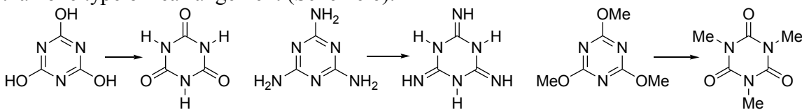
Scheme 5: The rearrangement of cyanuric acid, melamine, and trimethoxy triazine
