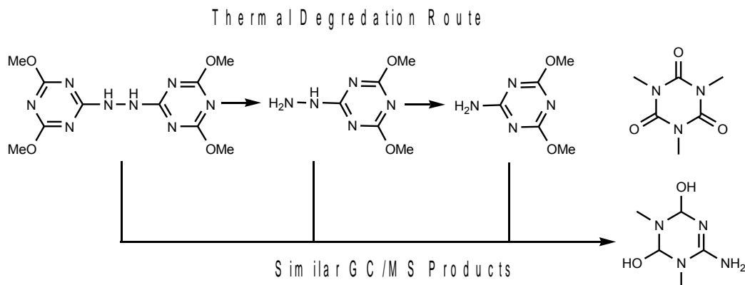
Scheme 4: Thermolysis products including rearrangement (1,3,5-trimethyl-1,3,5-triazinane-2,4,6-trione) and decay (6-amino-1,2,3,4-tetrahydro-1,3-dimethyl-1,3,5-triazine-2,4-diol) species.
