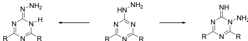
Scheme 6: Two possible rearrangement pathways for hydrazine substituents
