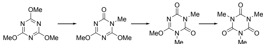
Scheme 2: Rearrangement accompanying methoxy substituents on triazine rings
